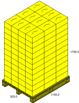
UK PALLET ( mm 1000 x 1200 x 144 )
